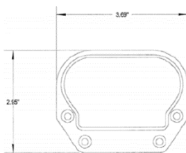
Collar
